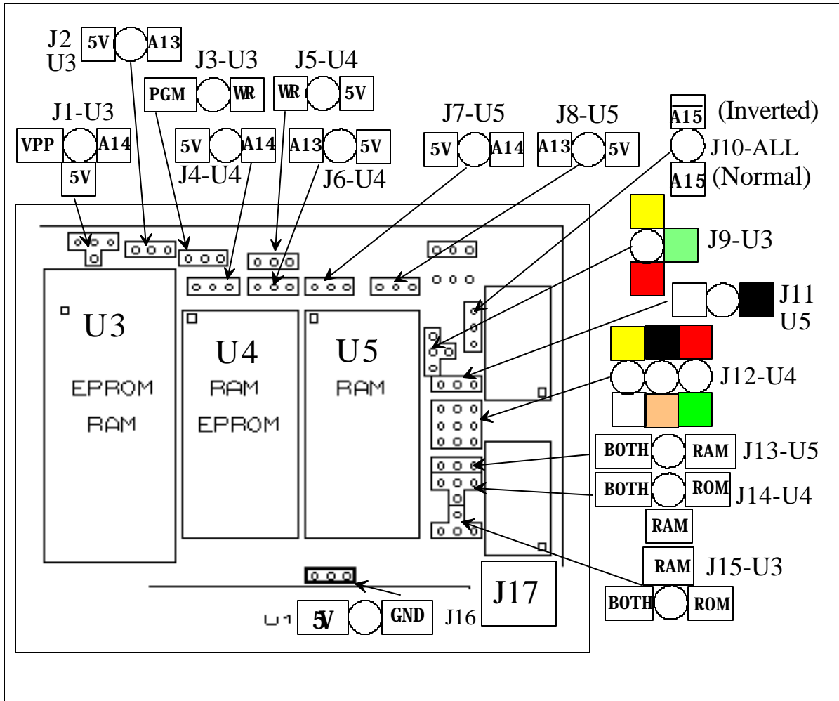
Memory Configuration Jumpers
