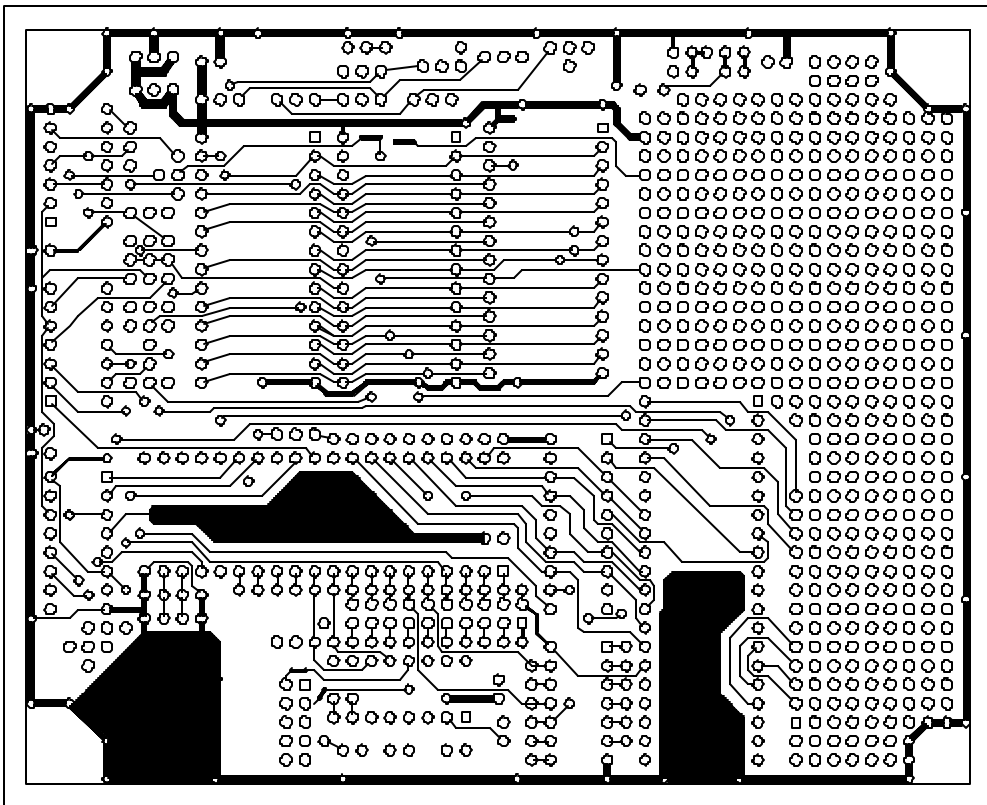
Solder side
