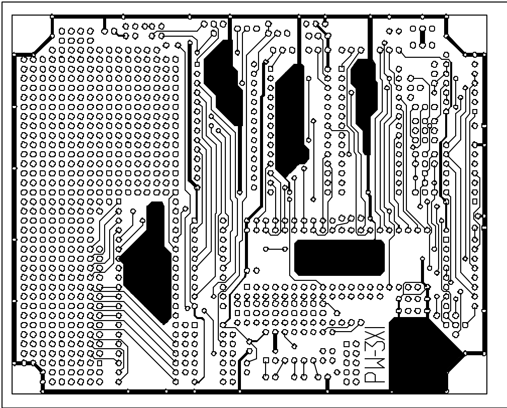
Component side ( □ = Pin 1 )
